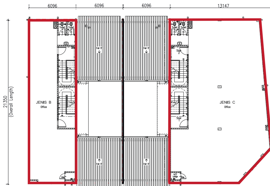
Second Floor
